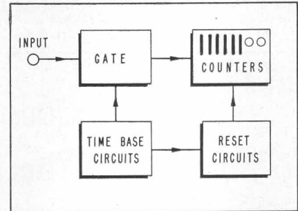
Fig. 4. Basic arrangement of counter circuits.
